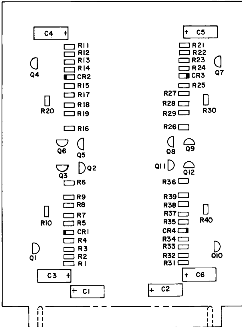
Figure 14. Circuit card assembly, L-2009 (Group 0).
