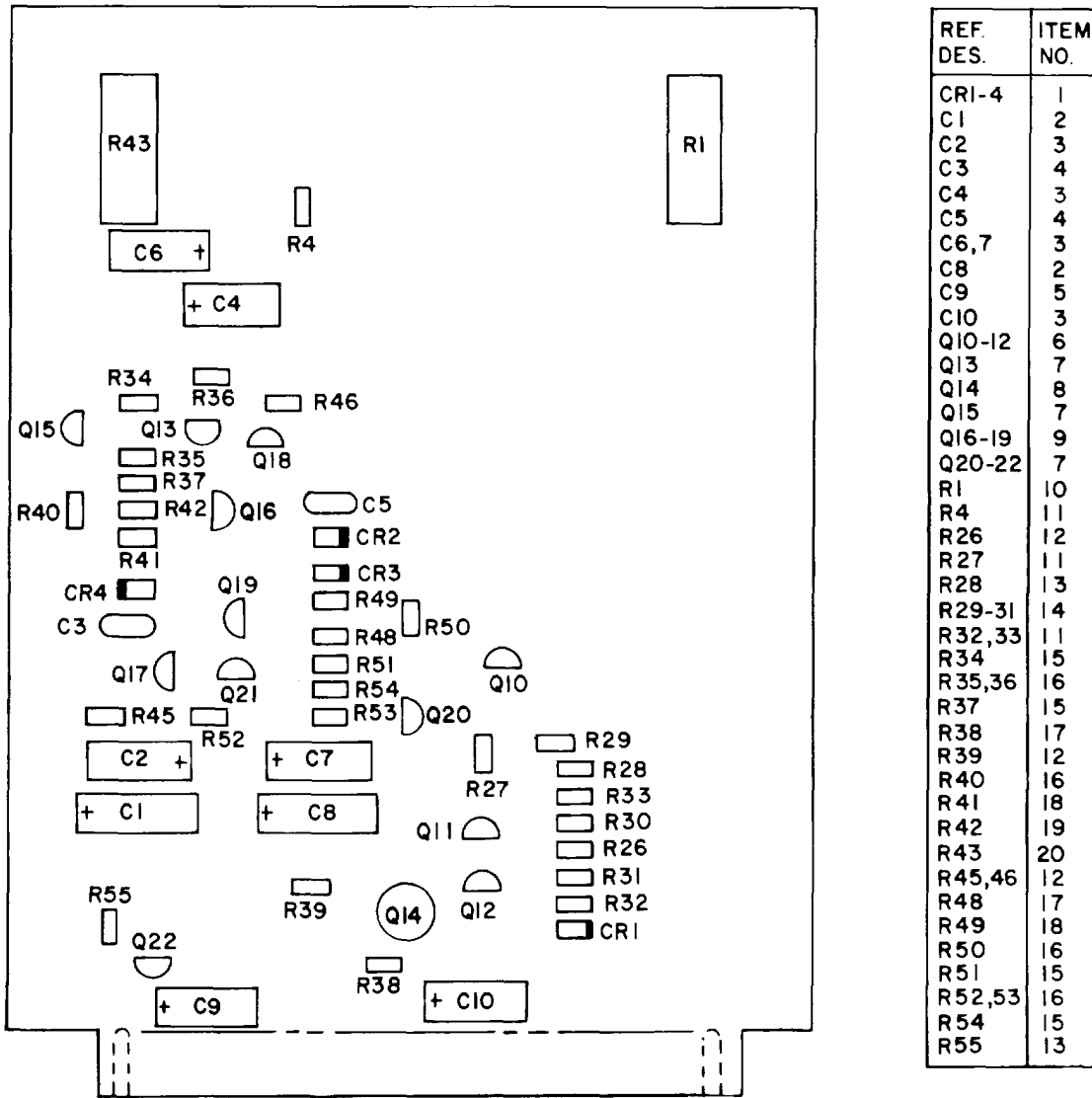
Figure 25. Circuit card assembly, L-2008 (Group 4A2).
