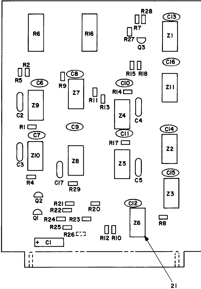
Figure 10. Circuit card assembly, L-2024 (Group 1).
