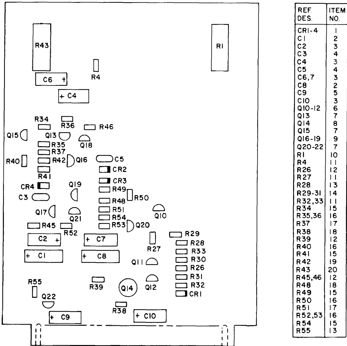
Figure 20. Circuit card assembly, L-2008 (Group 4B8).
