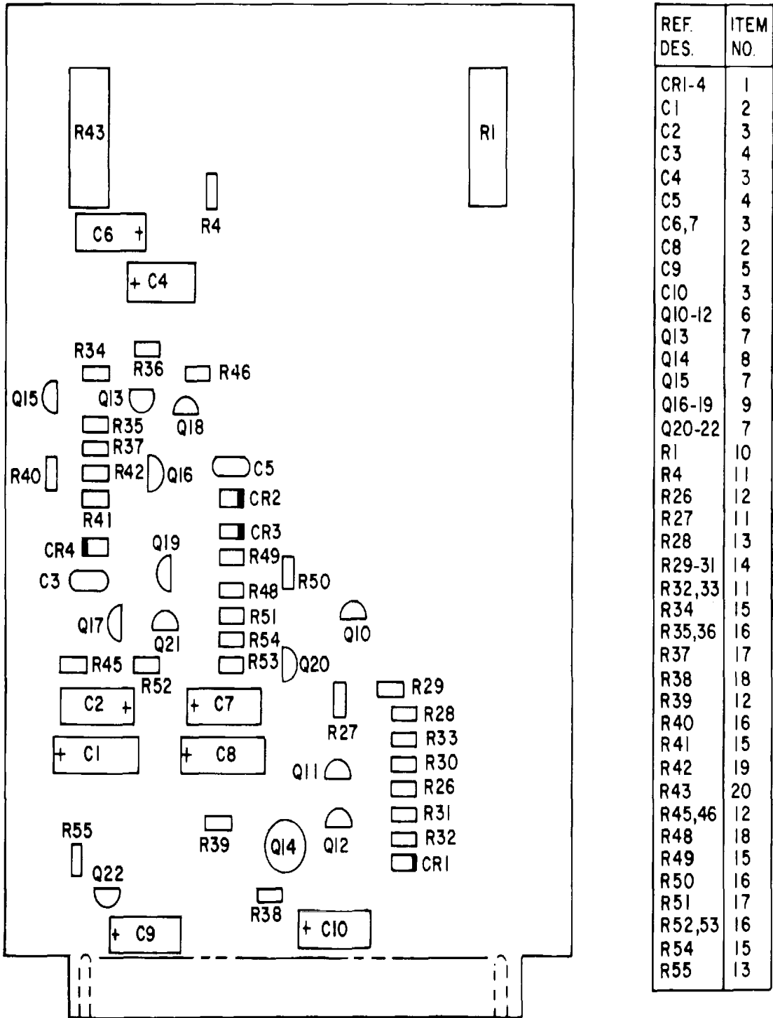
Figure 17. Circuit card assembly, L-2008 (Group 4B10).
