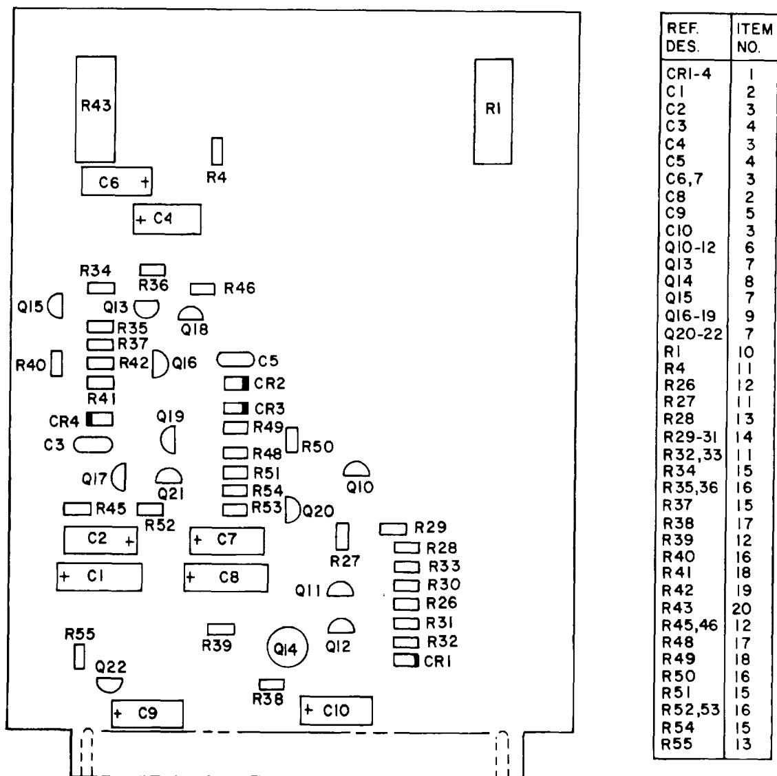
Figure 26. Circuit card assembly, L-2008 (Group 4A1).
