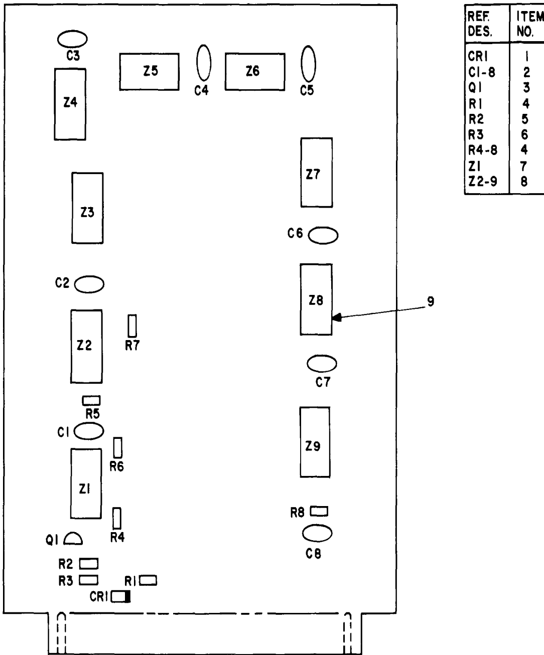
Figure 27. Circuit card assembly, L-2016 (Group 0).
