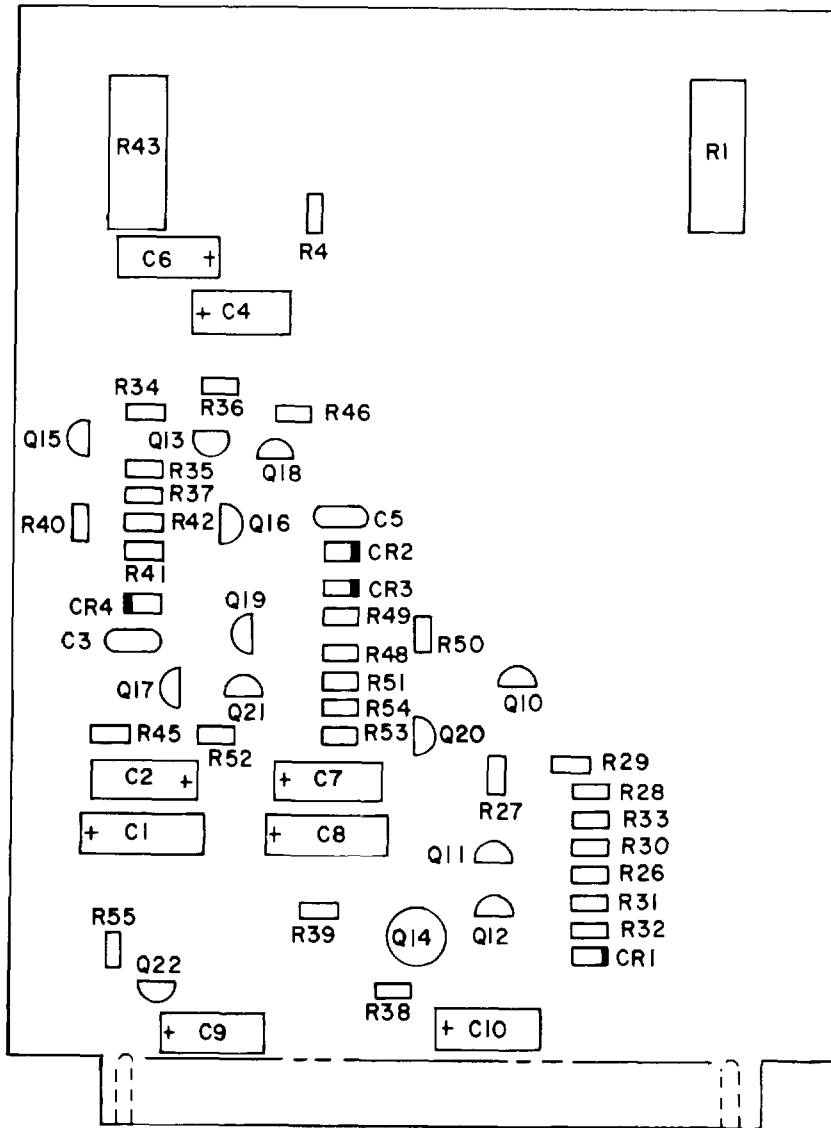
Figure 22. Circuit card assembly, L-2008 (Group 4A5).
