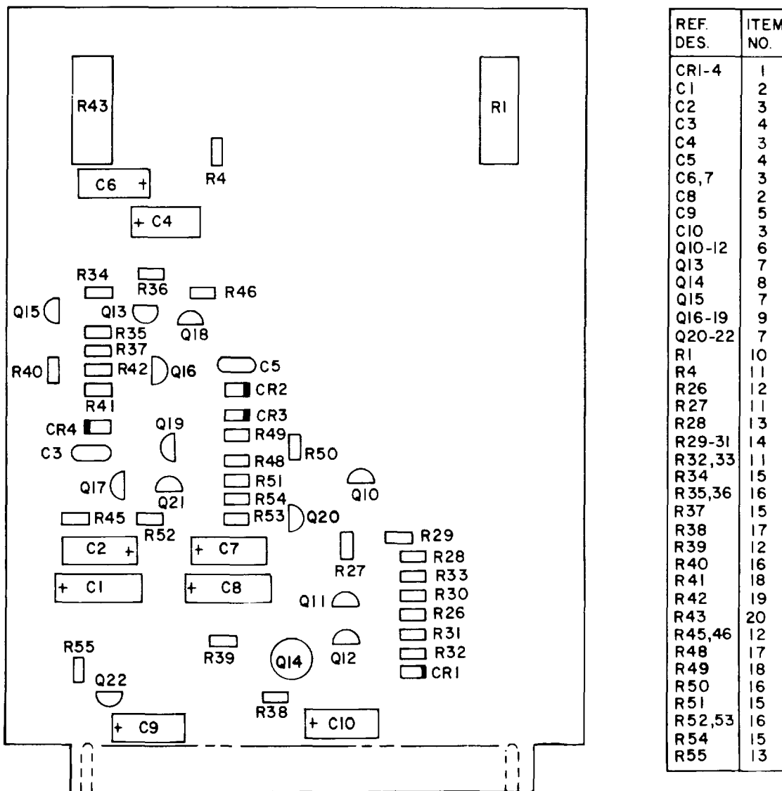
Figure 24. Circuit card assembly, L-2008 (Group 4A3).
