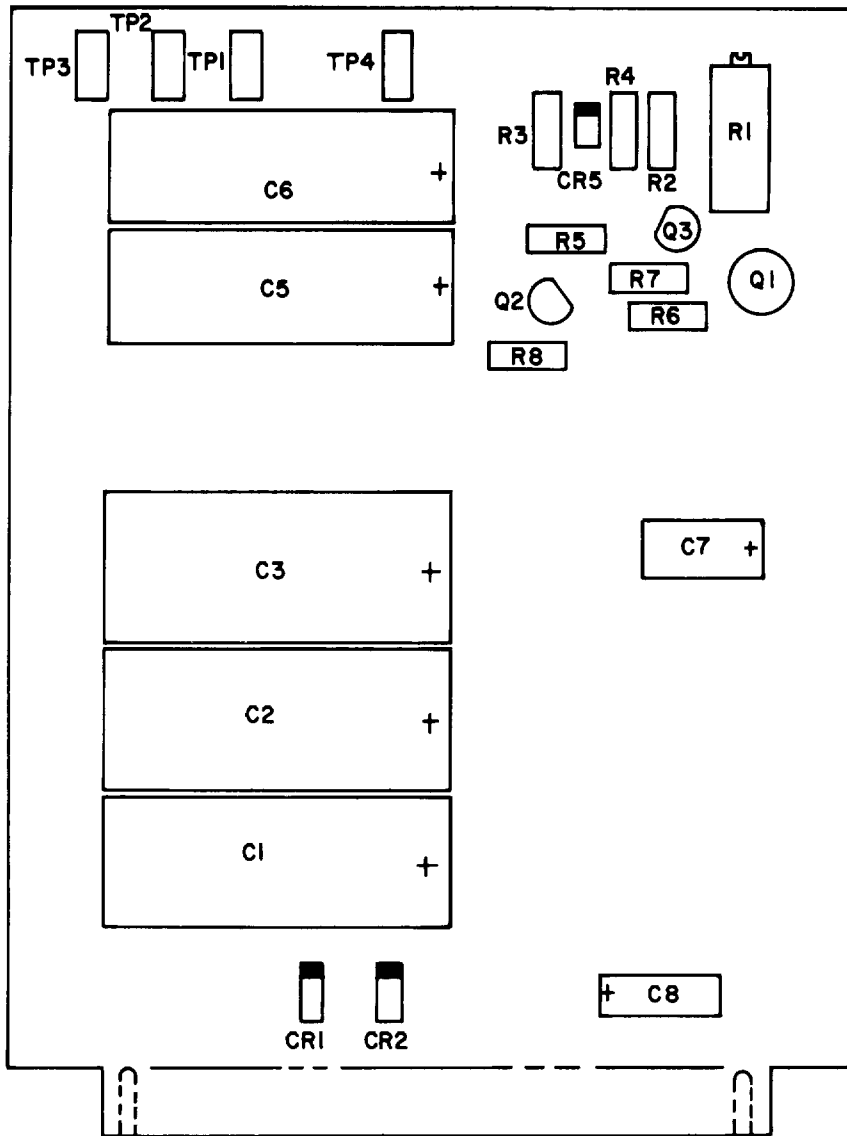
Figure 13. Circuit card assembly, L-2110 (Group 3).
