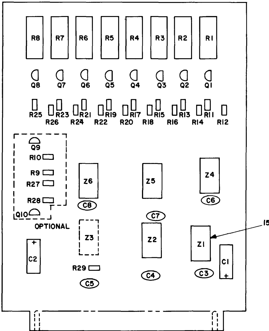
Figure 8. Circuit card assembly, L-2028 (Group 1).
