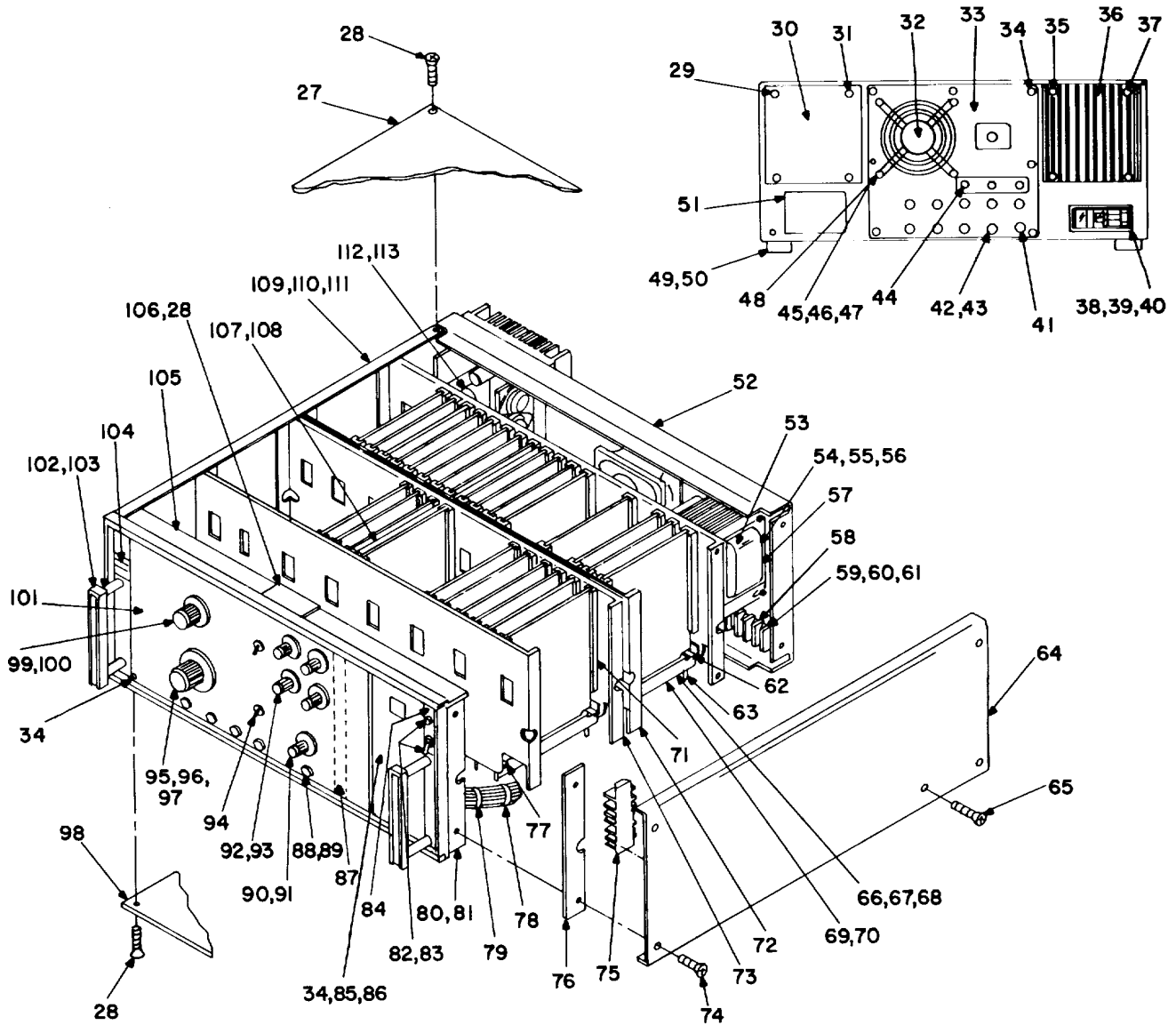
Figure 1. Test pattern generator SG-1223/T (Sheet 2 of 2).
